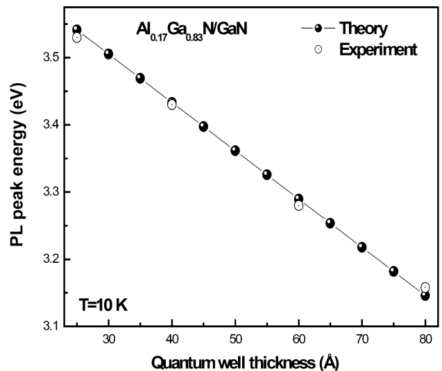
FIGURE 2. PL energy of \text{Al}_{0.17}\text{Ga}_{0.83}\text{N}/\text{GaN} QWs as a function of the well width. The experimental data are well accounted for by Eq. (8) taking into account an internal electric field of 719 KV/cm.
