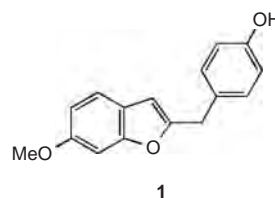
Scheme 1.
