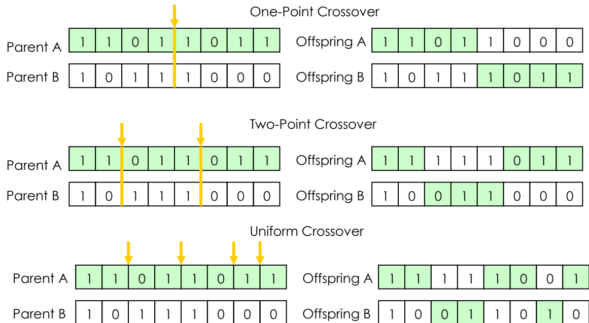
Figure 3.2 – Crossover operators.
